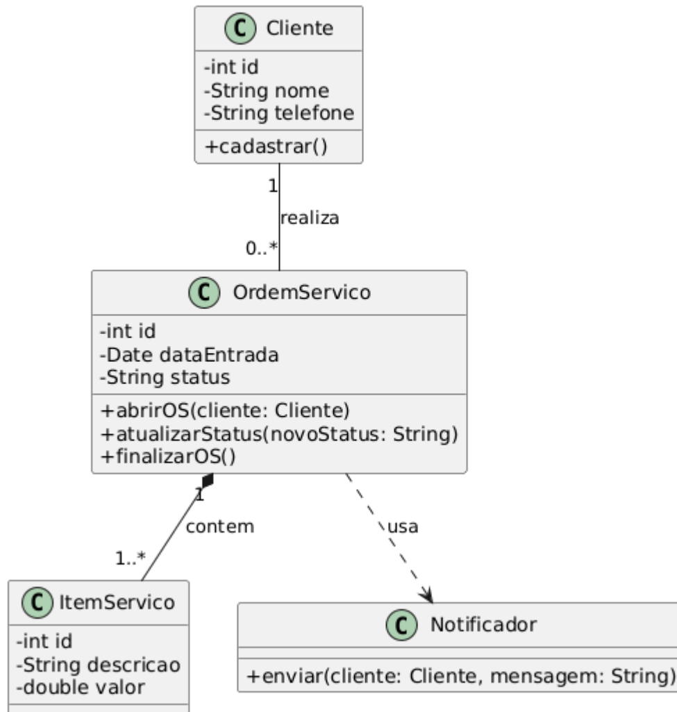
Diagrama de Classes - Lavanderia Express
